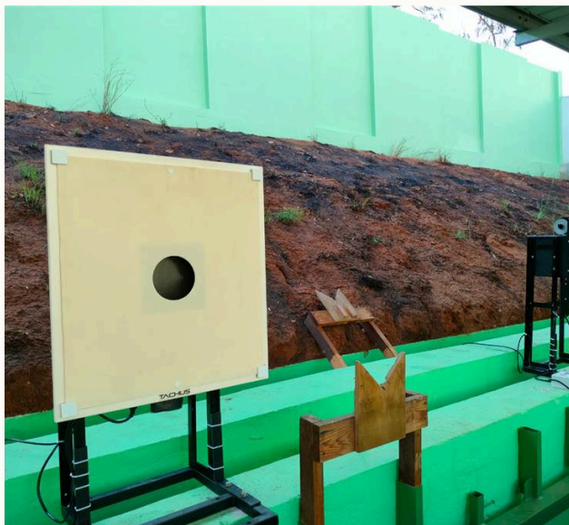
Tachus 50/10 ETS units on their stands at a covered range Fig. 01
